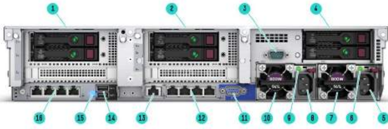
Rear View – With optional FlexLOM, Rear drives and Serial port shown.
