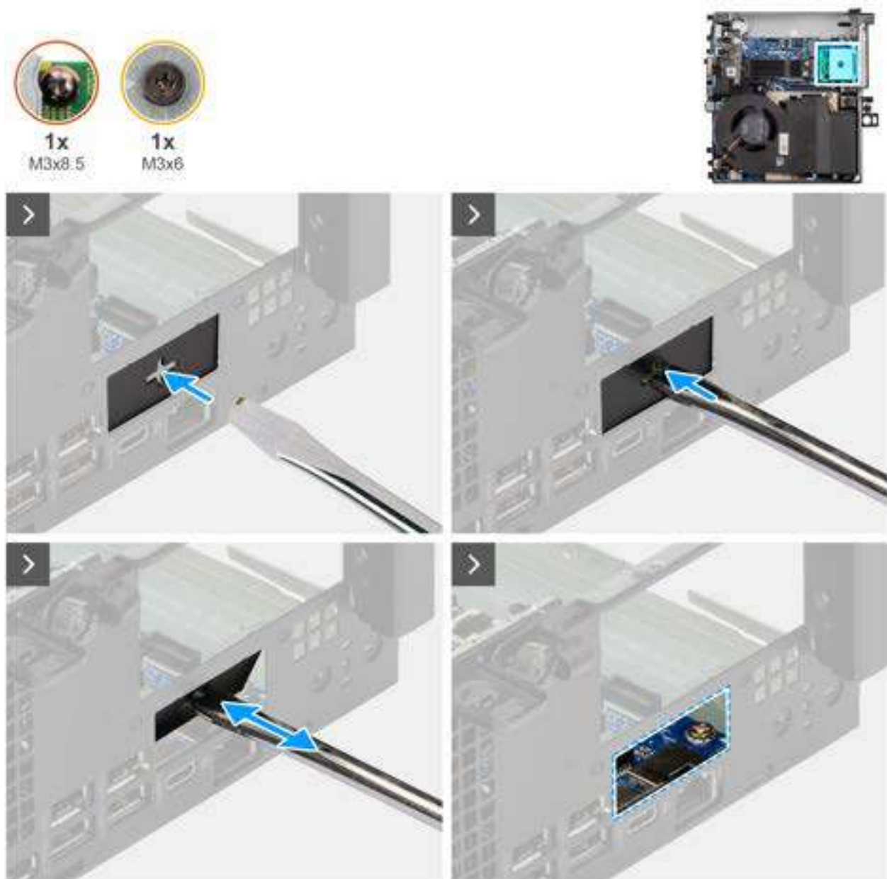
Figure 41. Installation du port Thunderbolt
