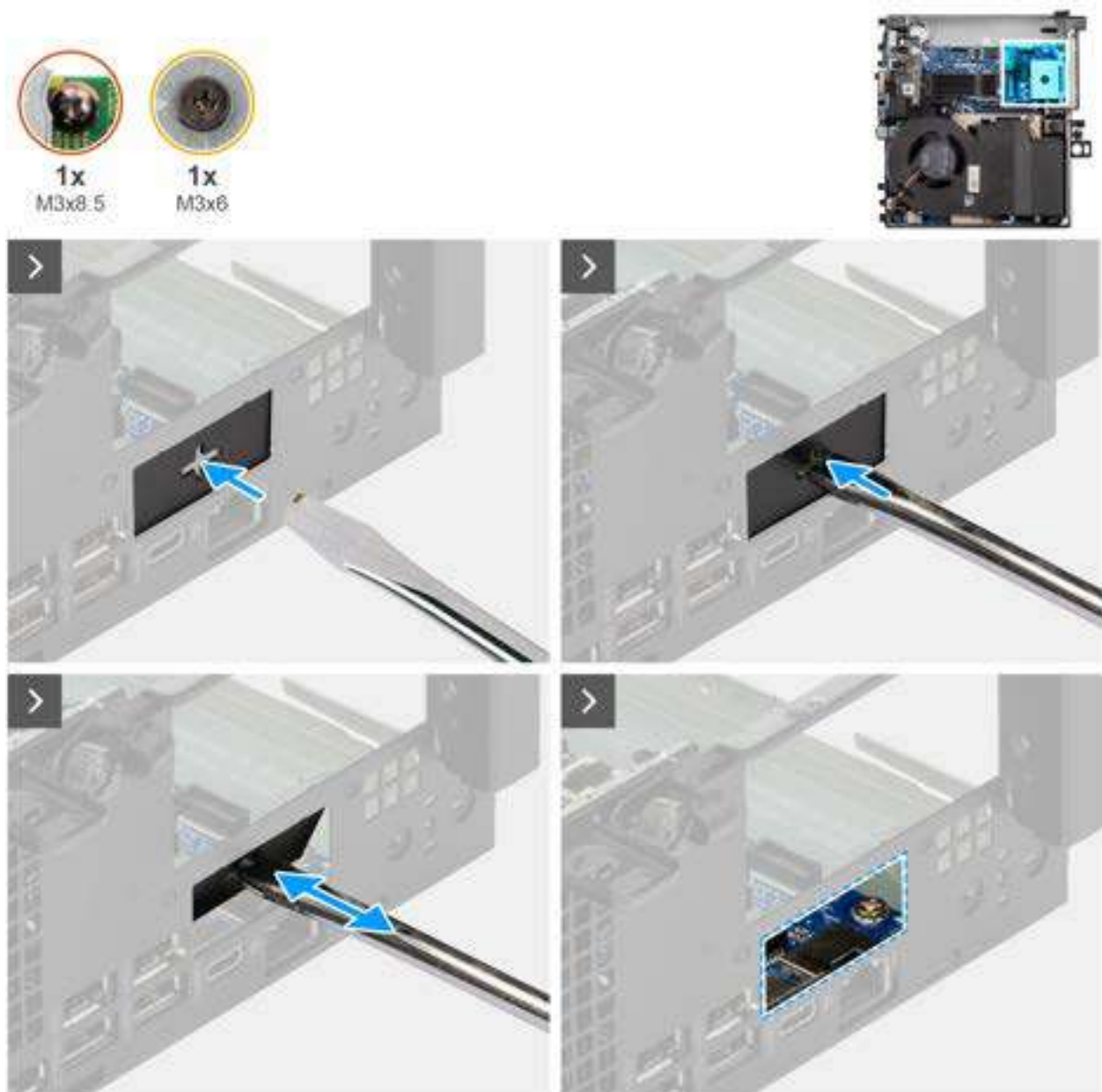
Figure 35. Installation du port PS2
