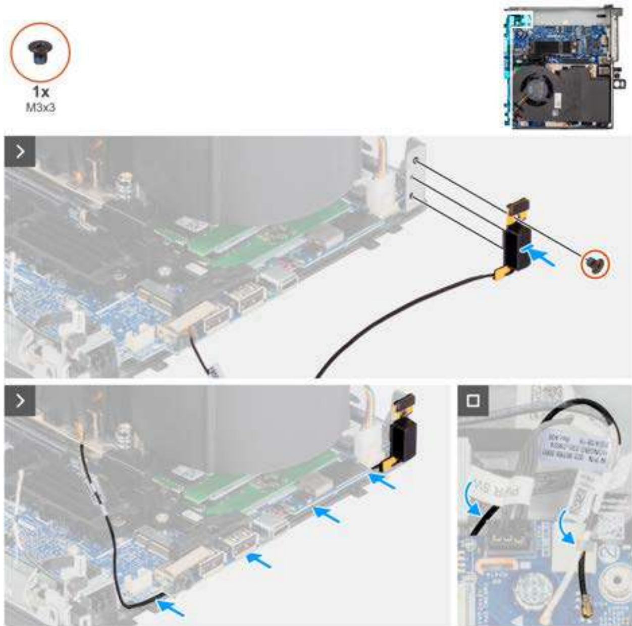
Figure 62. Installation de l'antenne interne (emplacement 2)
